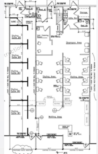
SECOND FLOOR 1,494 SF
